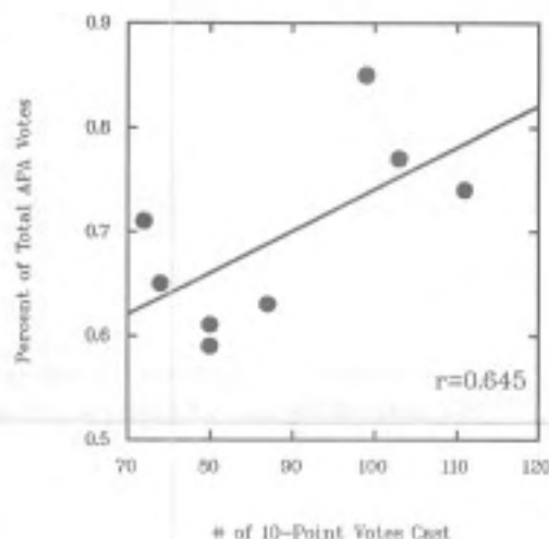
Fig. 2. Correlation of 10-point votes with % of total APA votes, 1983-90.
